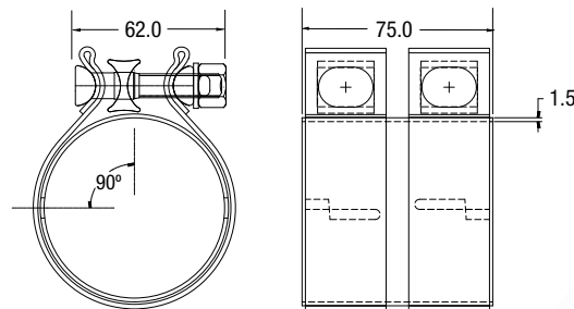
Units: mm
