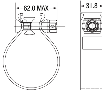
Units: mm
